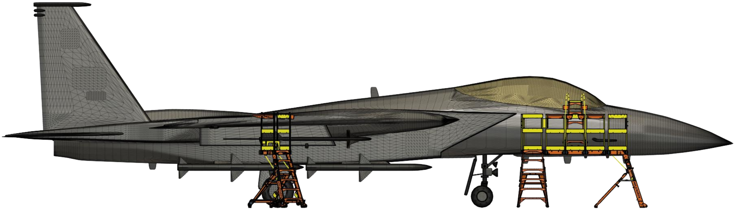
MX5+SD (MX5+ Service Deck, includes optional Retractable Wheel Kit- RWK)
